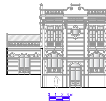
Elevation 03
